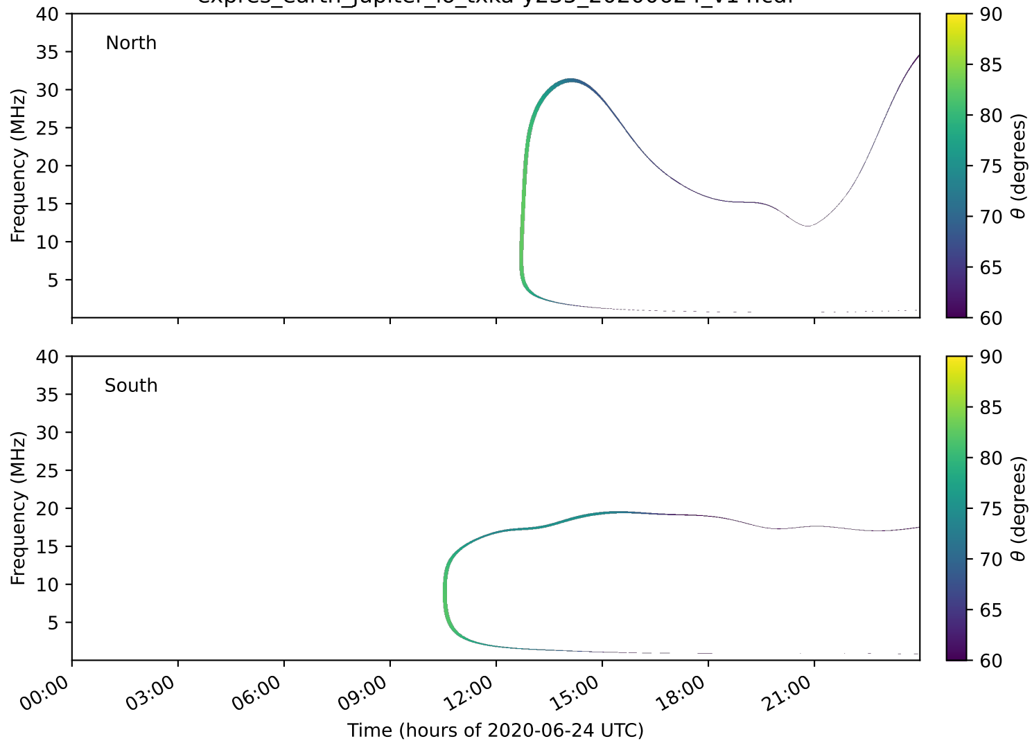
expres_earth_jupiter_io_txka-y235_20200624_v14.cdf
