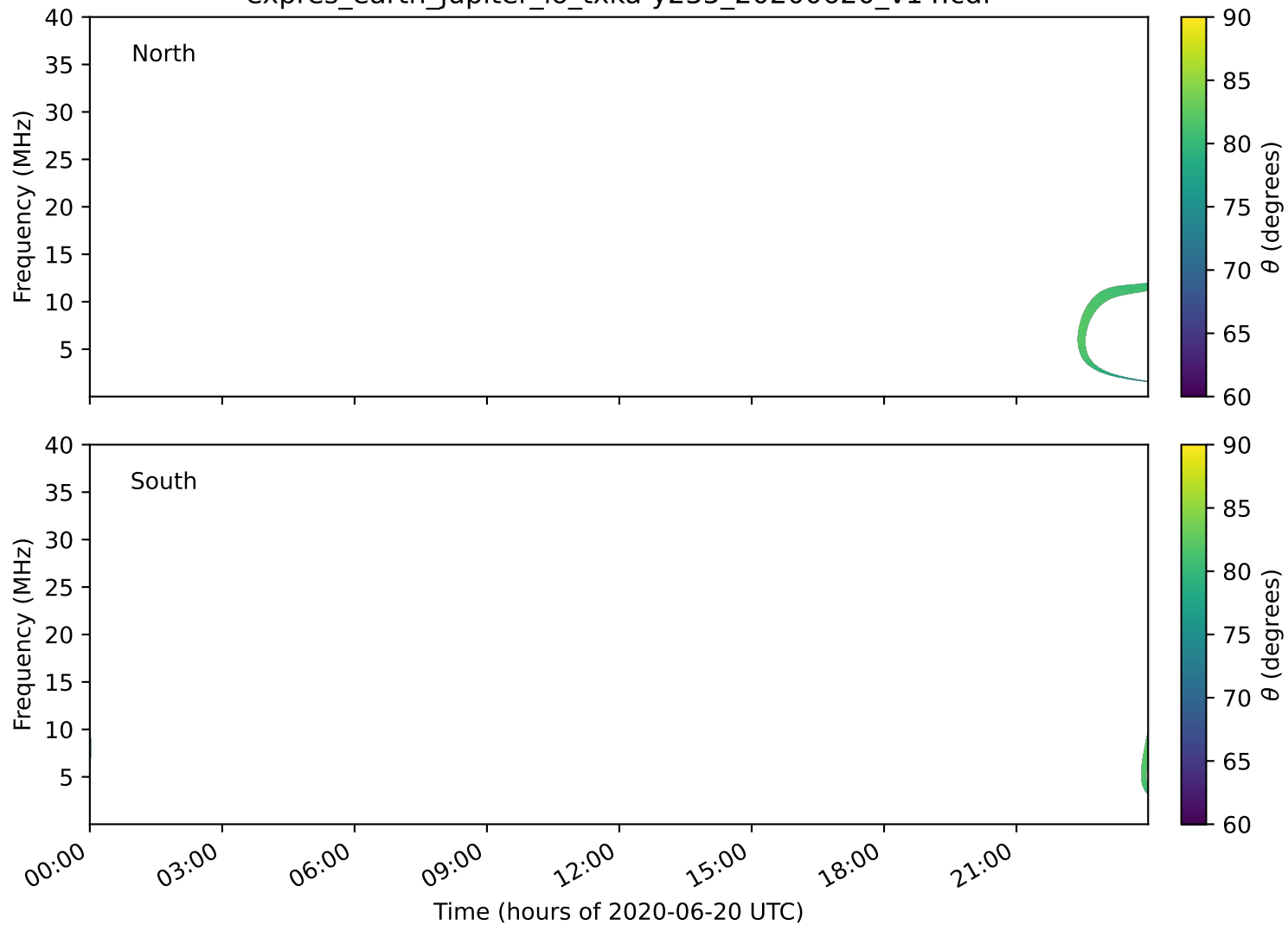
expres_earth_jupiter_io_txka-y235_20200620_v14.cdf
