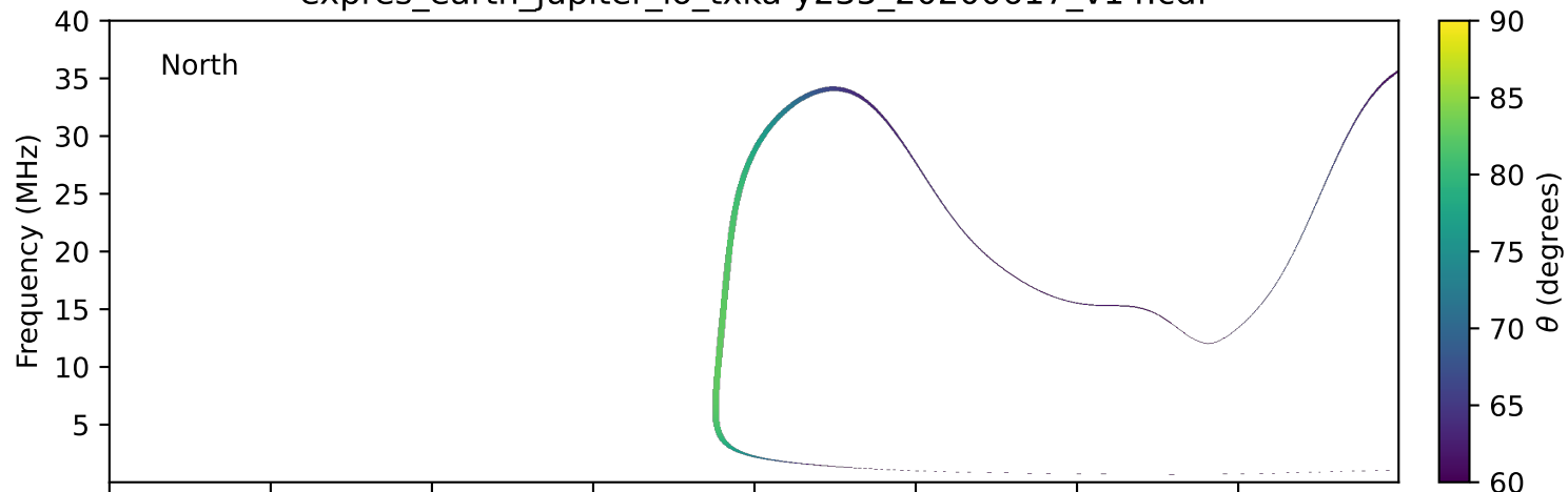
expres_earth_jupiter_io_txka-y235_20200617_v14.cdf
