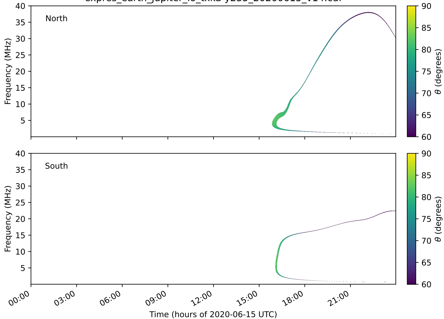
expres_earth_jupiter_io_txka-y235_20200615_v14.cdf
