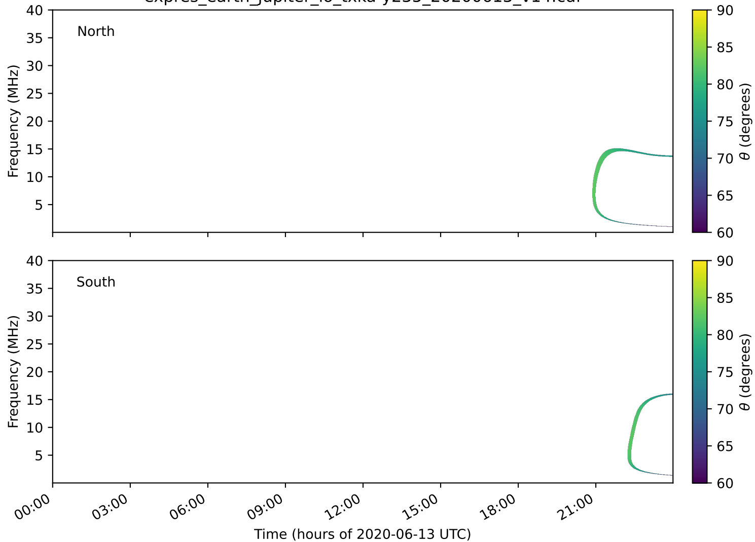
expres_earth_jupiter_io_txka-y235_20200613_v14.cdf
