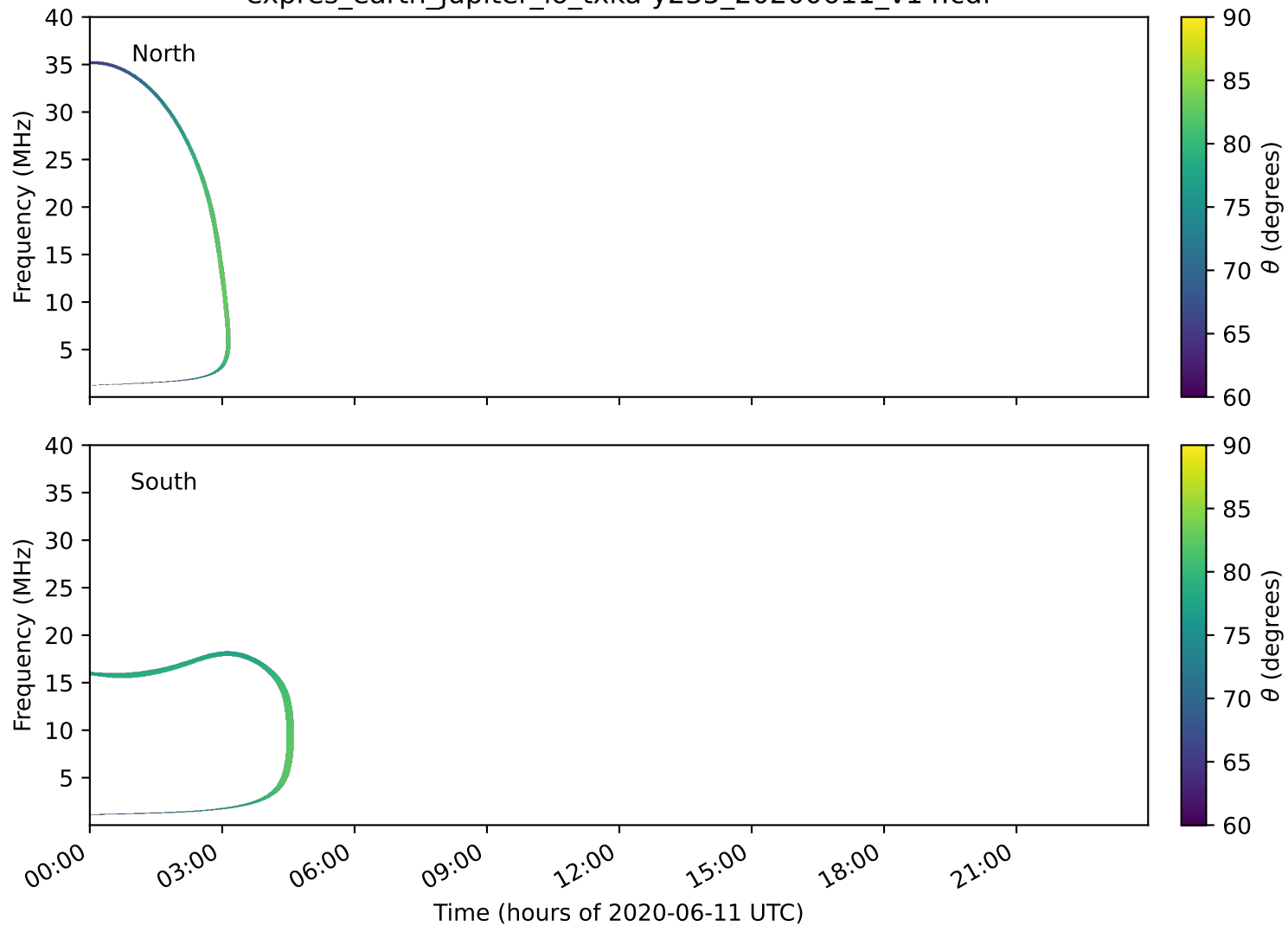
expres_earth_jupiter_io_txka-y235_20200611_v14.cdf
