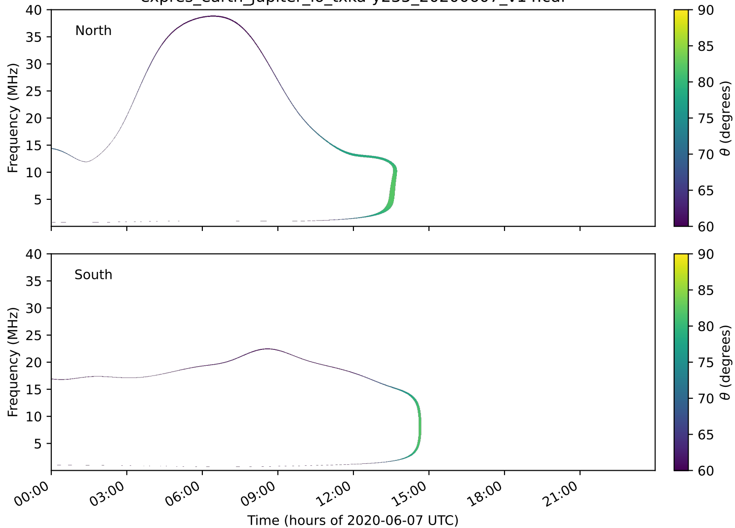
expres_earth_jupiter_io_txka-y235_20200607_v14.cdf
