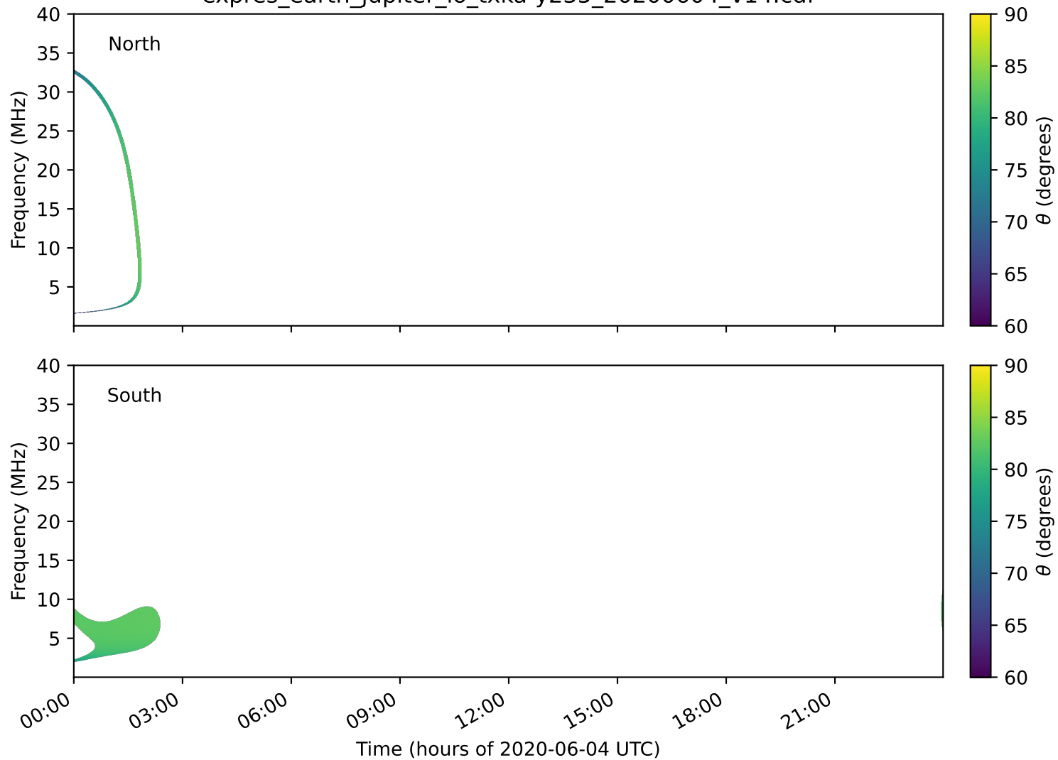
expres_earth_jupiter_io_txka-y235_20200604_v14.cdf
