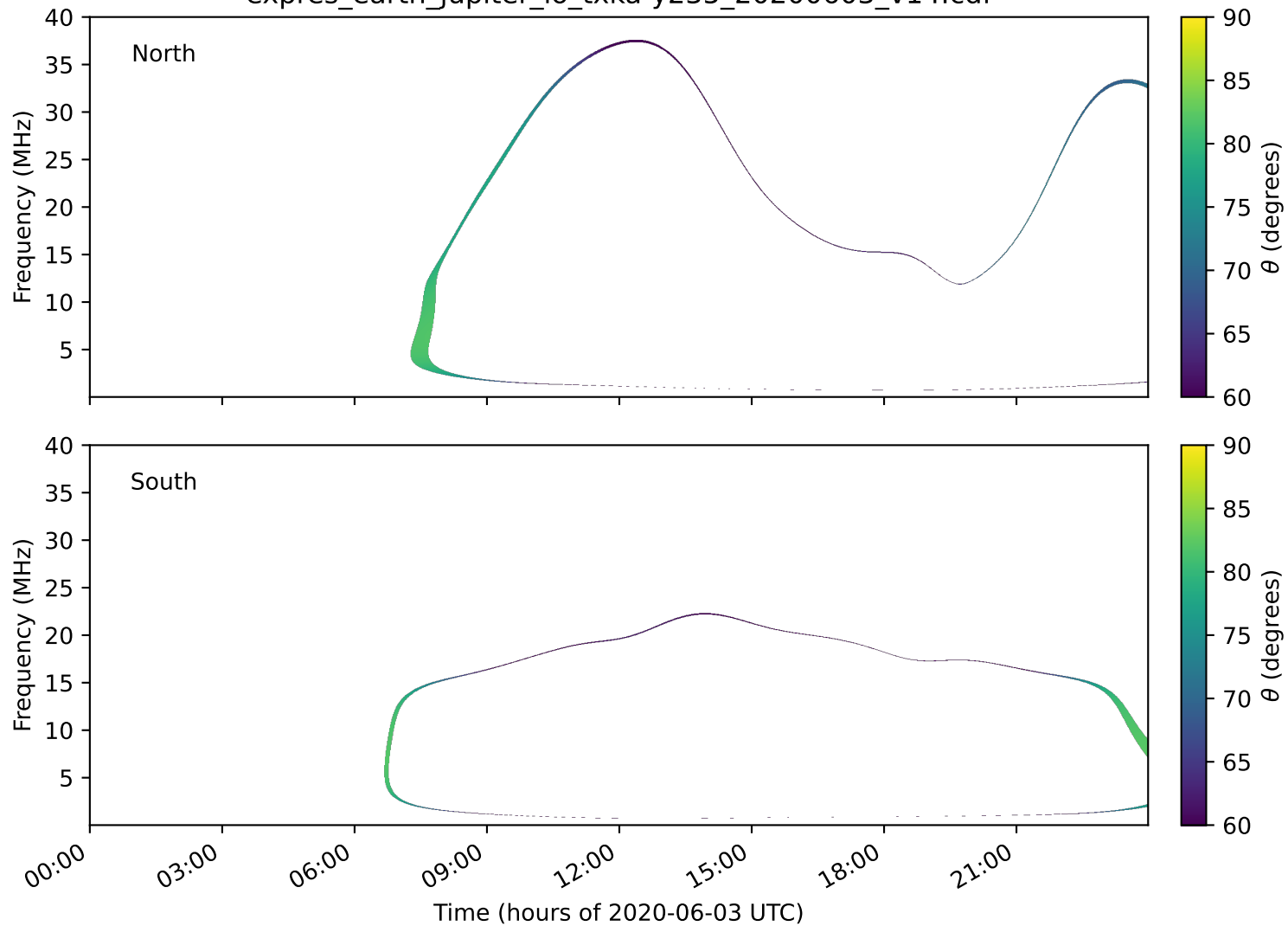
expres_earth_jupiter_io_txka-y235_20200603_v14.cdf
