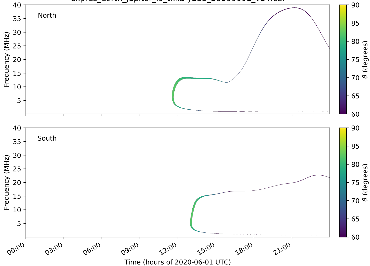
expres_earth_jupiter_io_txka-y235_20200601_v14.cdf
