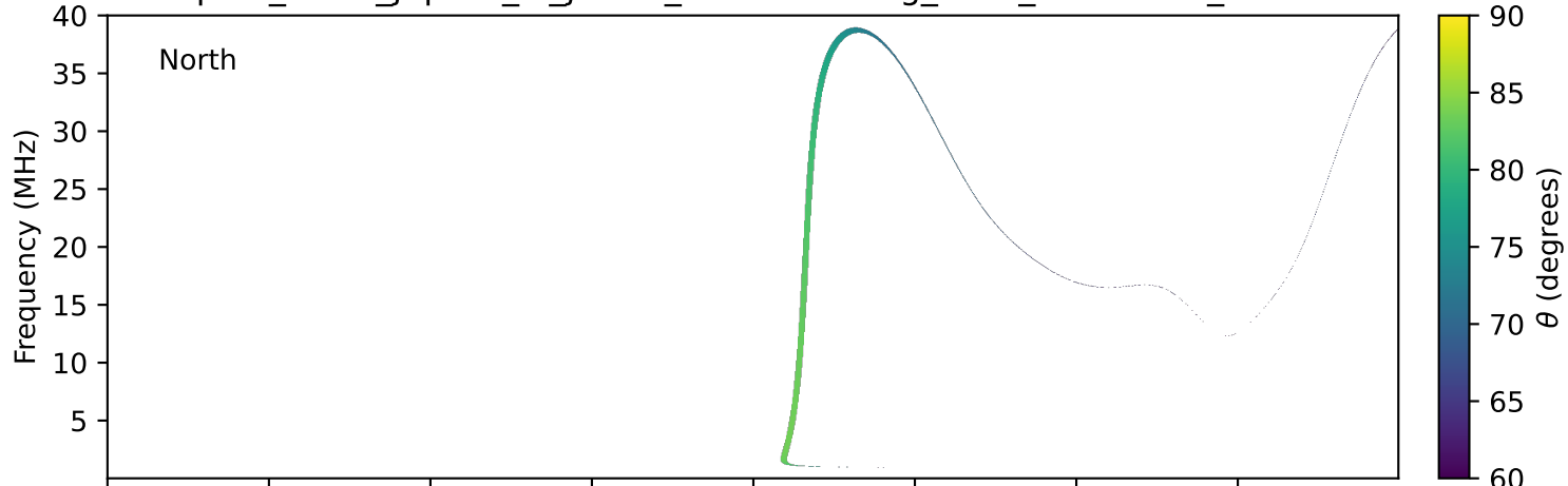
expres_earth_jupiter_io_jrm33_lossc-wid1deg_3kev_20200624_v11.cdf
