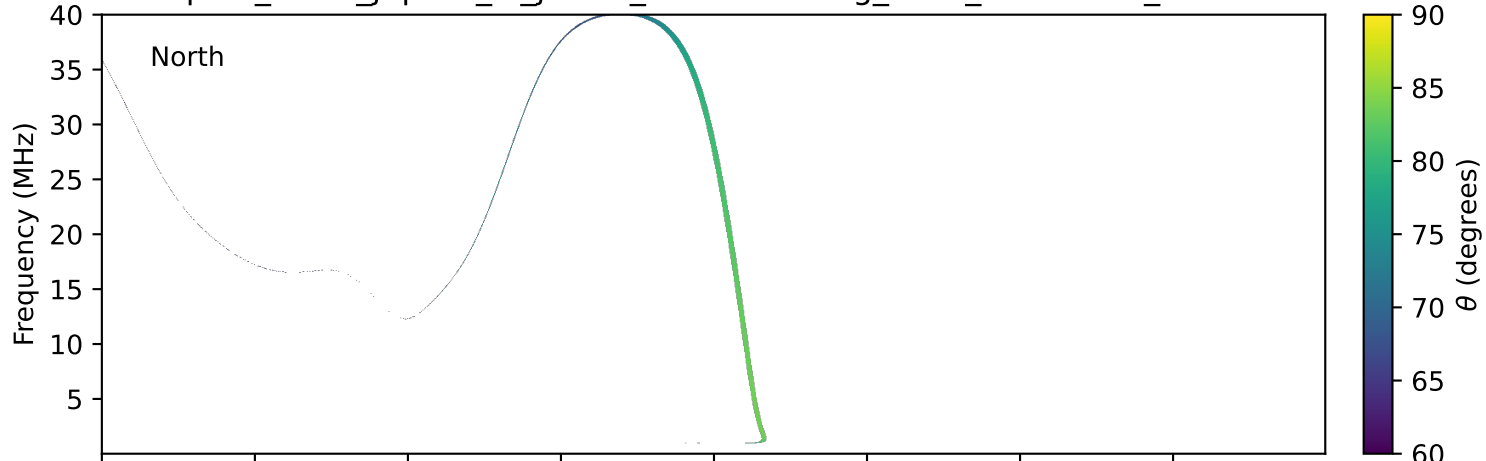
expres_earth_jupiter_io_jrm33_lossc-wid1deg_3kev_20200623_v11.cdf
