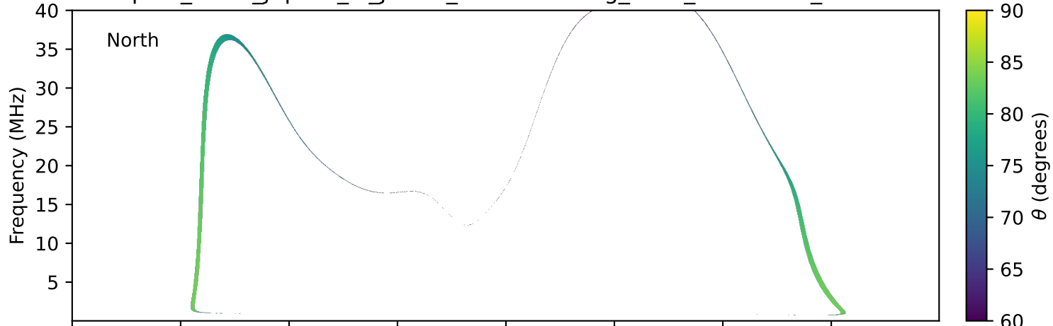
expres_earth_jupiter_io_jrm33_lossc-wid1deg_3kev_20200612_v11.cdf
