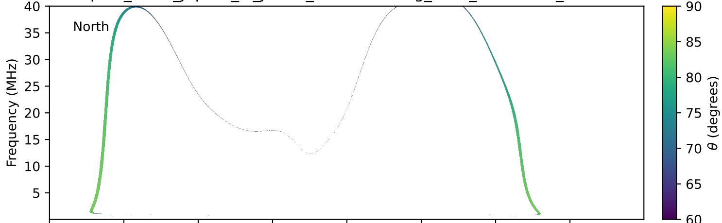
expres_earth_jupiter_io_jrm33_lossc-wid1deg_3kev_20200605_v11.cdf
