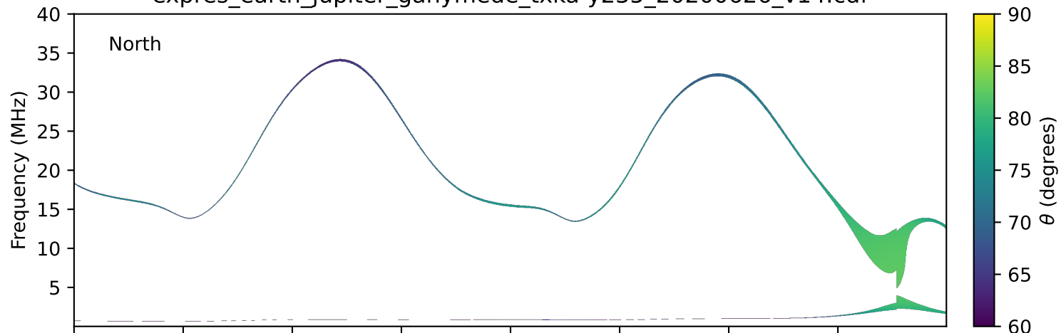
expres_earth_jupiter_ganymede_txka-y235_20200626_v14.cdf
