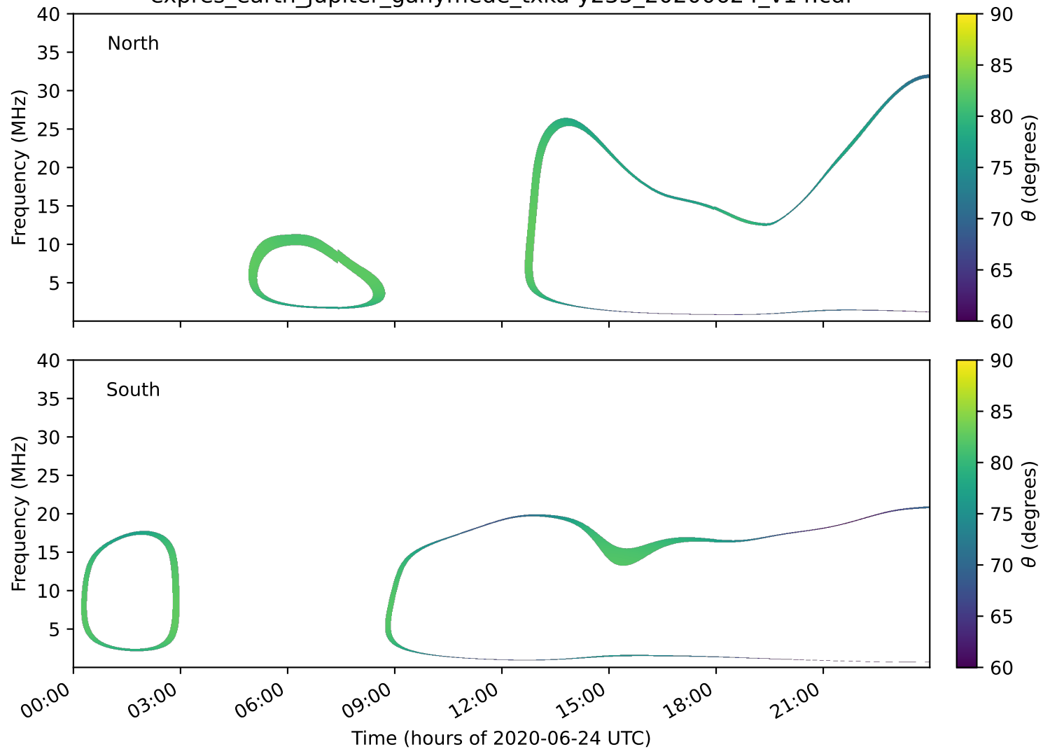
expres_earth_jupiter_ganymede_txka-y235_20200624_v14.cdf
