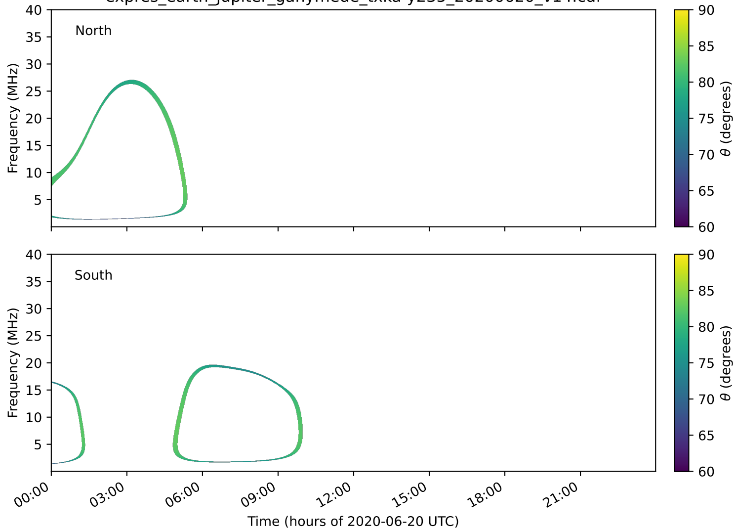
expres_earth_jupiter_ganymede_txka-y235_20200620_v14.cdf
