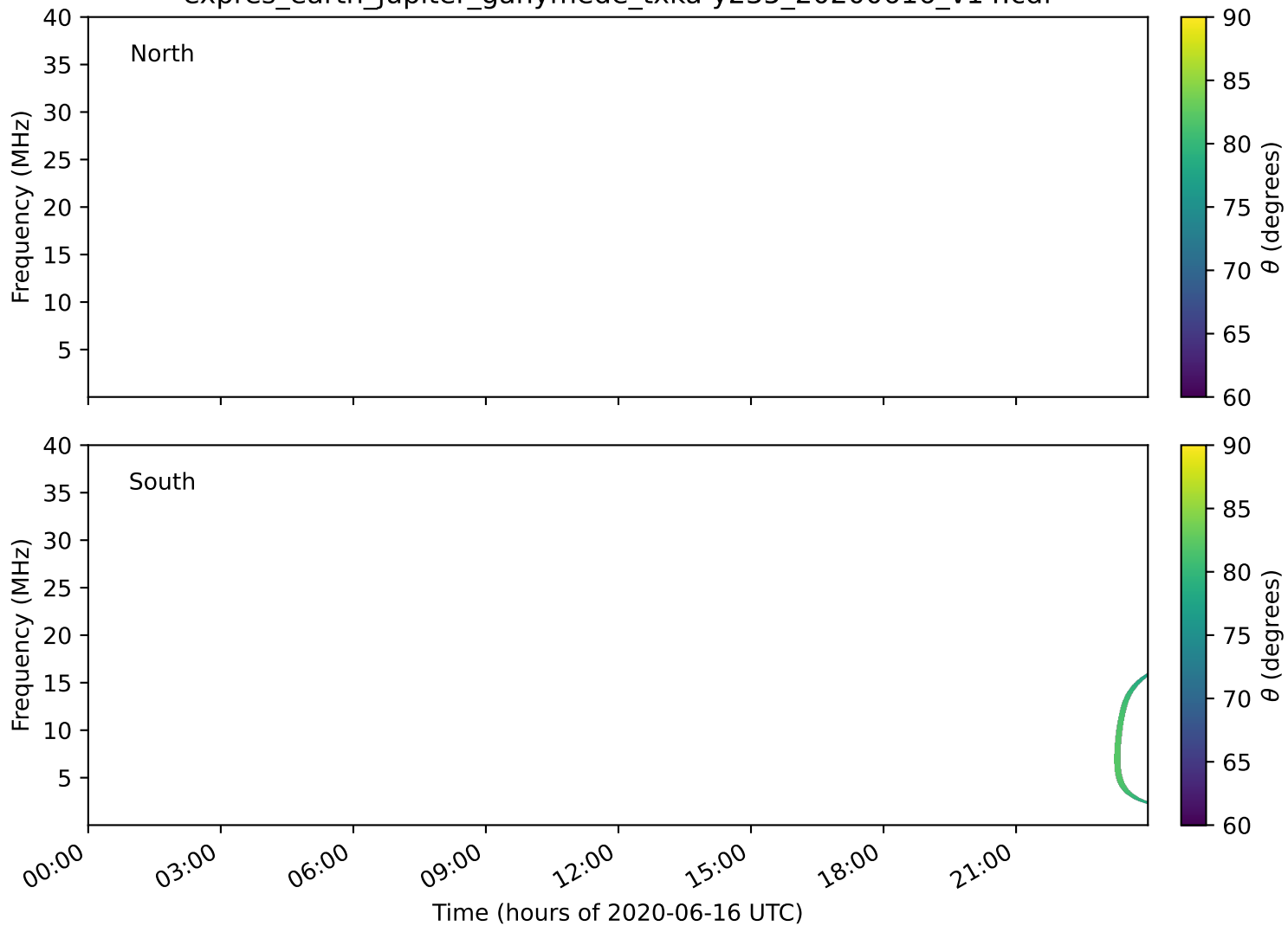
expres_earth_jupiter_ganymede_txka-y235_20200616_v14.cdf
