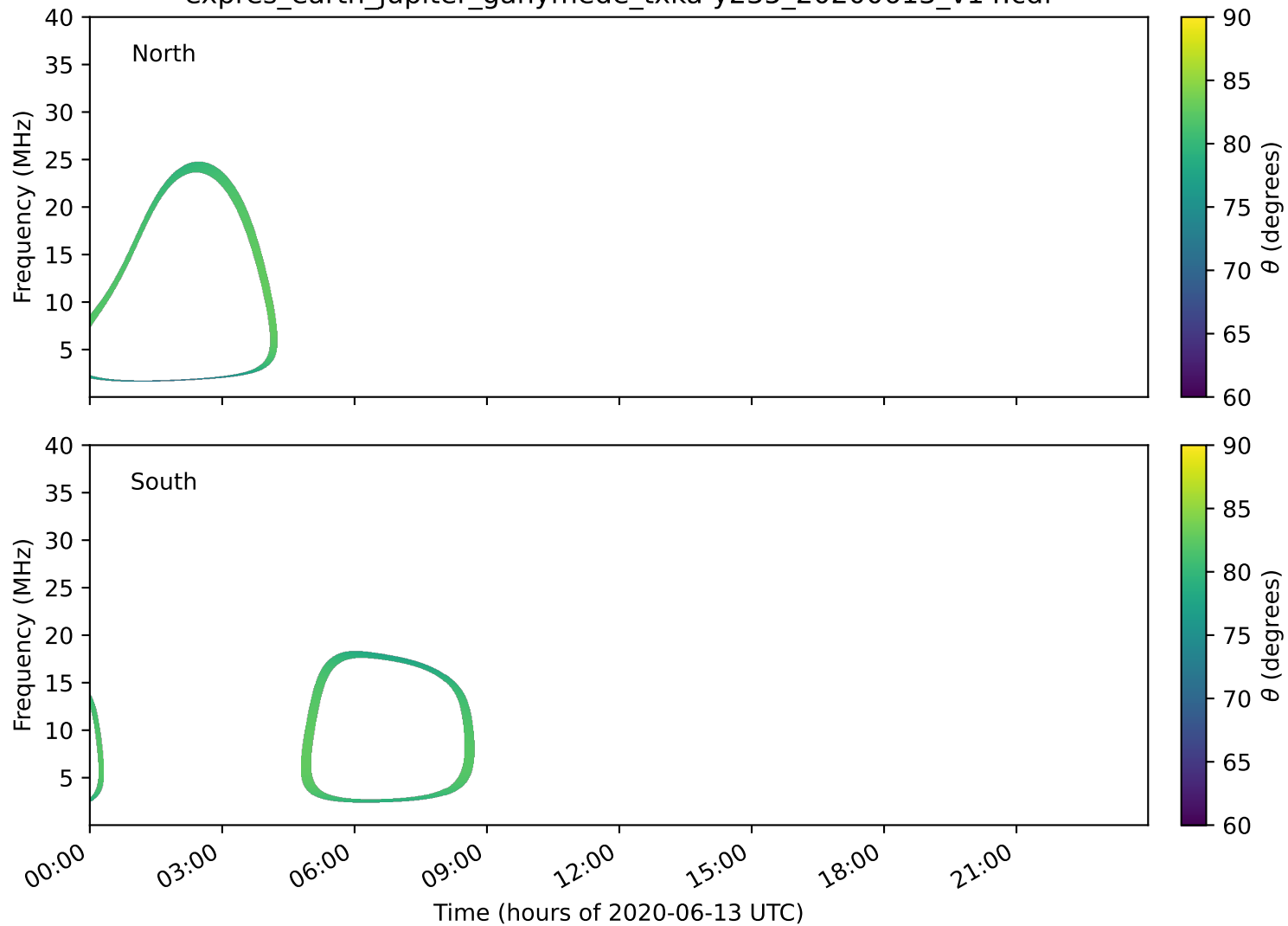
expres_earth_jupiter_ganymede_txka-y235_20200613_v14.cdf
