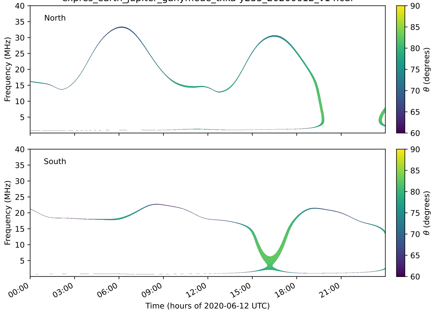
expres_earth_jupiter_ganymede_txka-y235_20200612_v14.cdf
