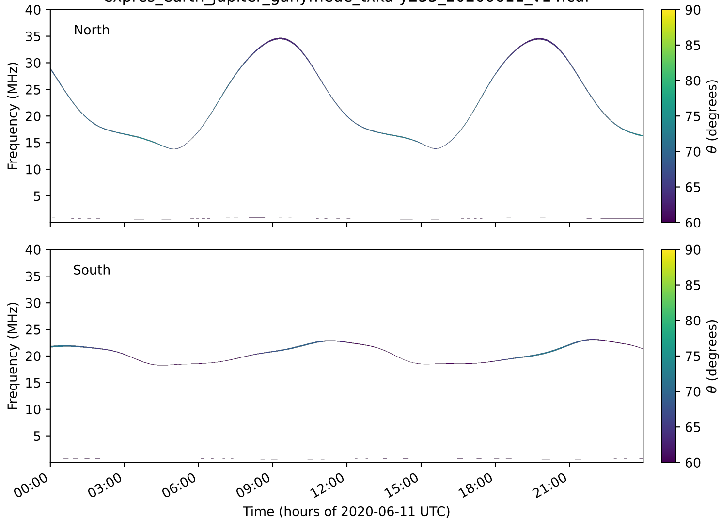
expres_earth_jupiter_ganymede_txka-y235_20200611_v14.cdf
