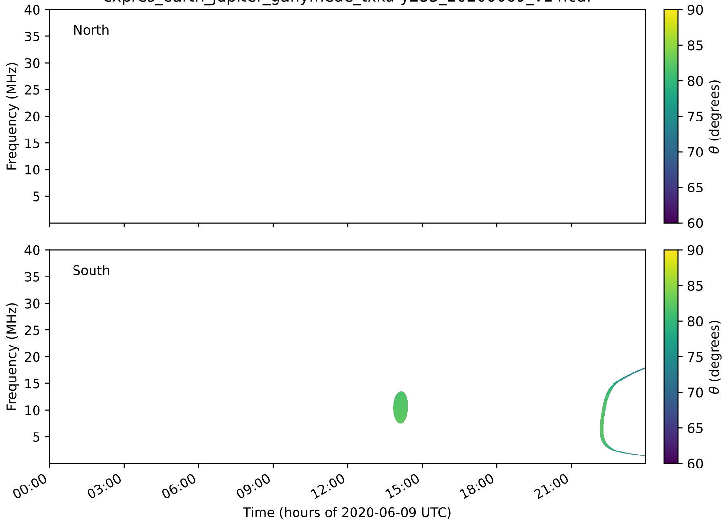
expres_earth_jupiter_ganymede_txka-y235_20200609_v14.cdf
