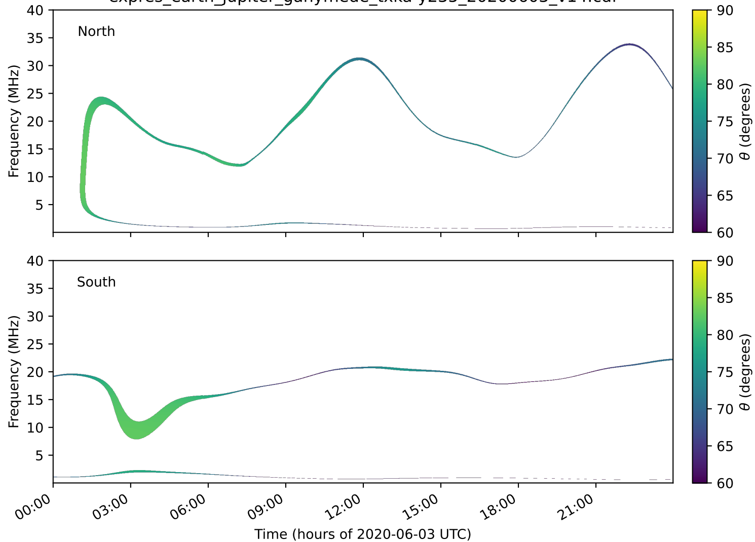
expres_earth_jupiter_ganymede_txka-y235_20200603_v14.cdf
