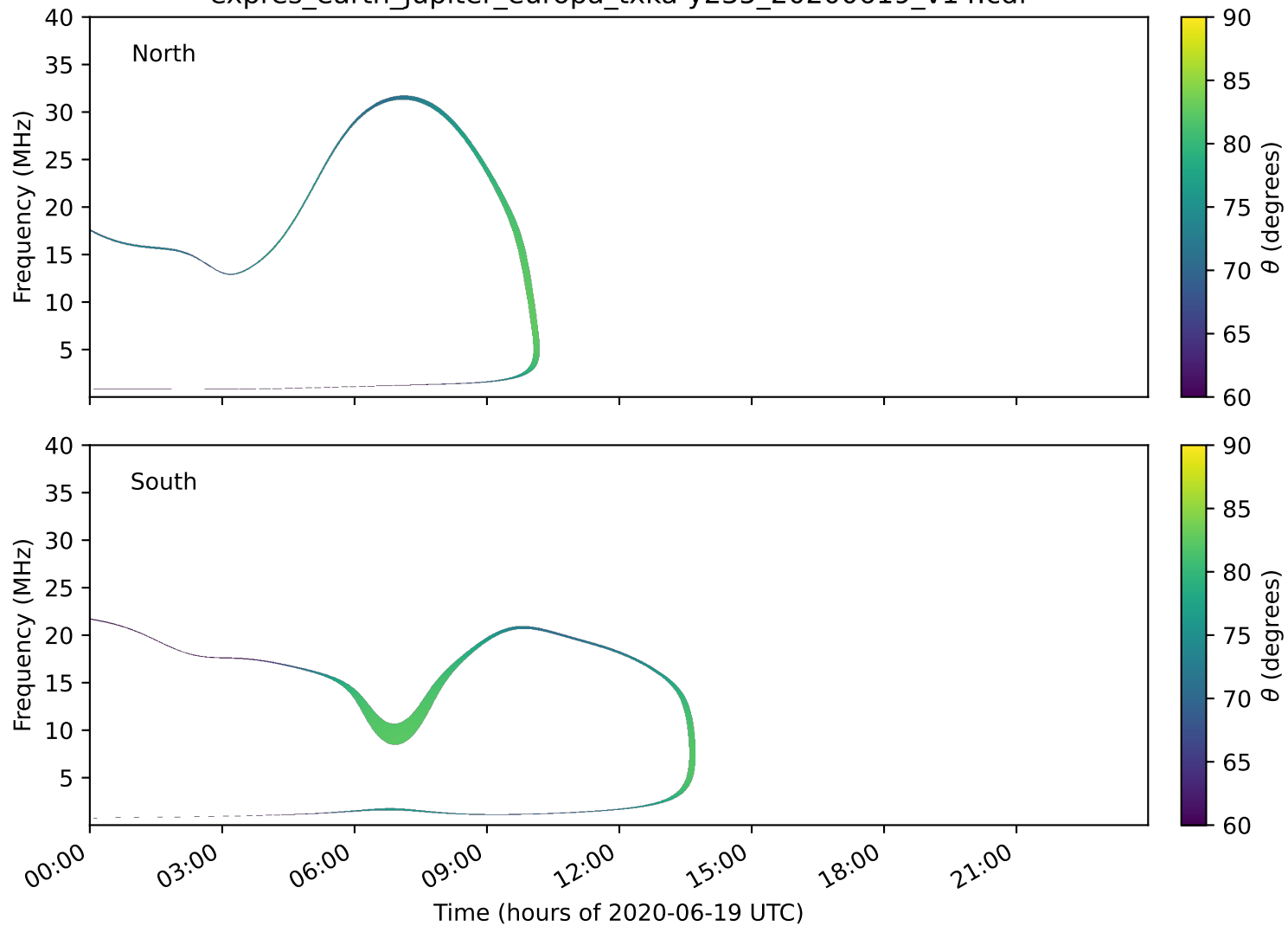
expres_earth_jupiter_europa_txka-y235_20200619_v14.cdf
