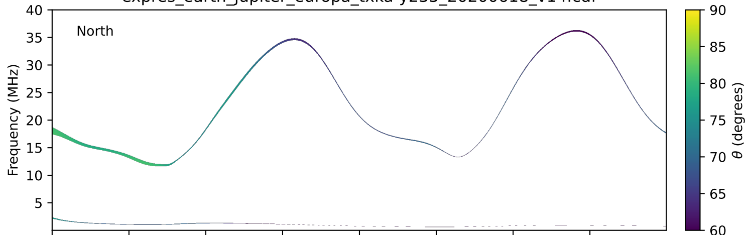
expres_earth_jupiter_europa_txka-y235_20200618_v14.cdf
