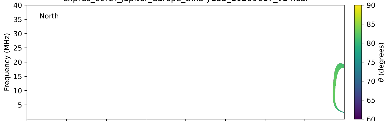
expres_earth_jupiter_europa_txka-y235_20200617_v14.cdf
