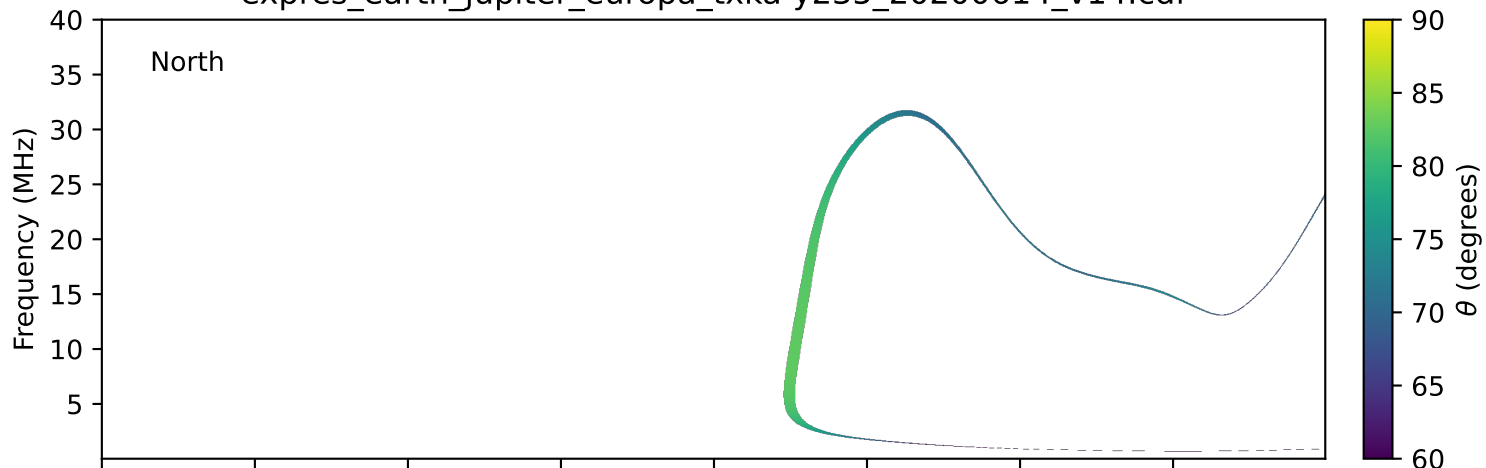
expres_earth_jupiter_europa_txka-y235_20200614_v14.cdf
