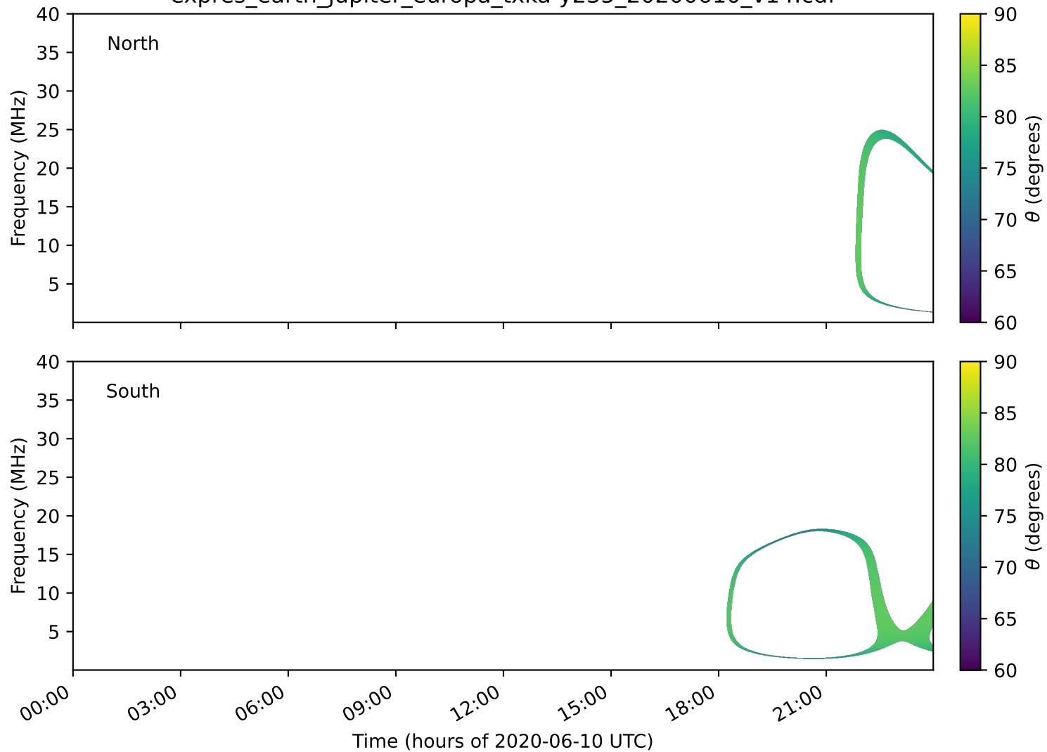
expres_earth_jupiter_europa_txka-y235_20200610_v14.cdf
