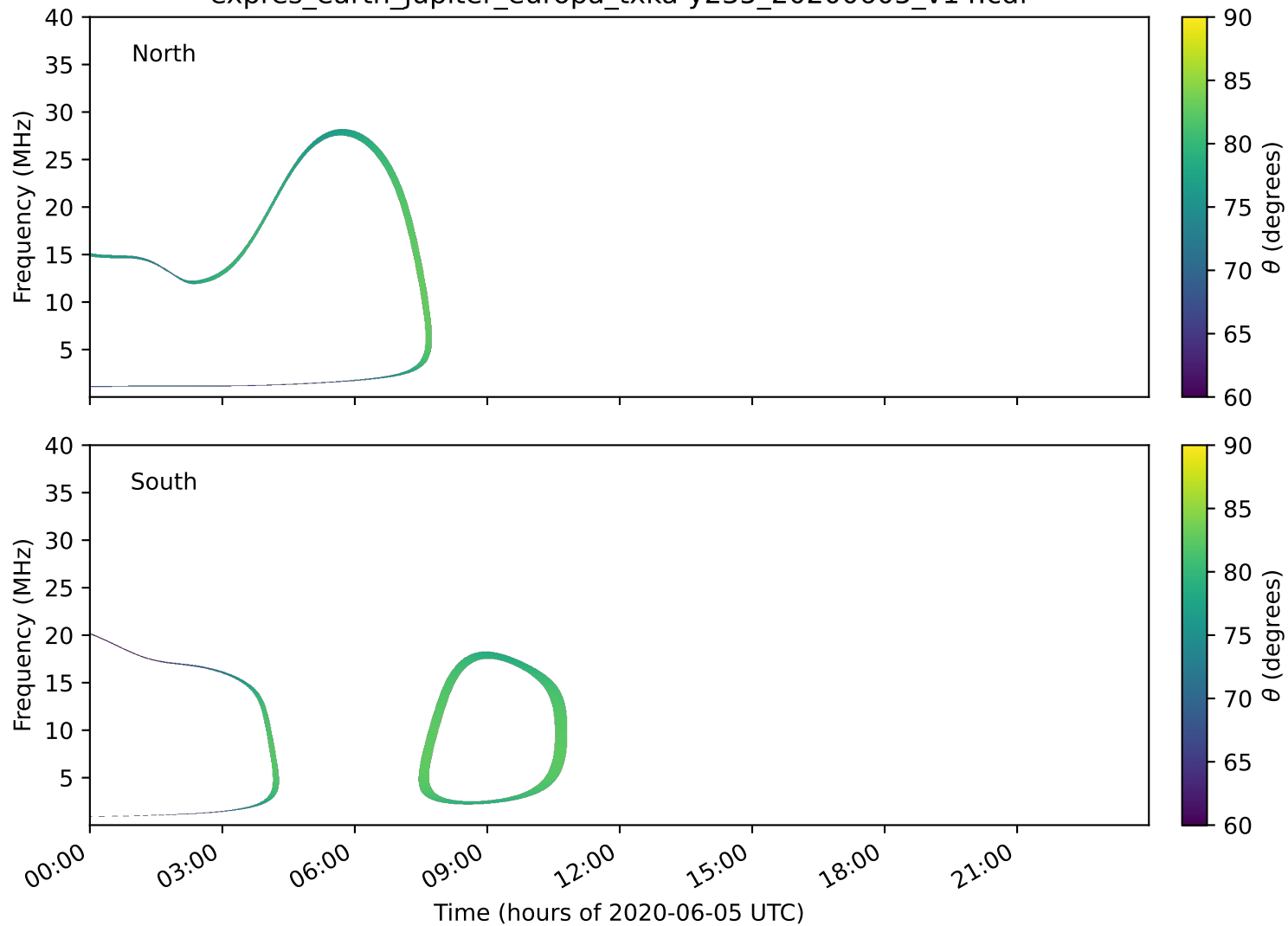
expres_earth_jupiter_europa_txka-y235_20200605_v14.cdf
