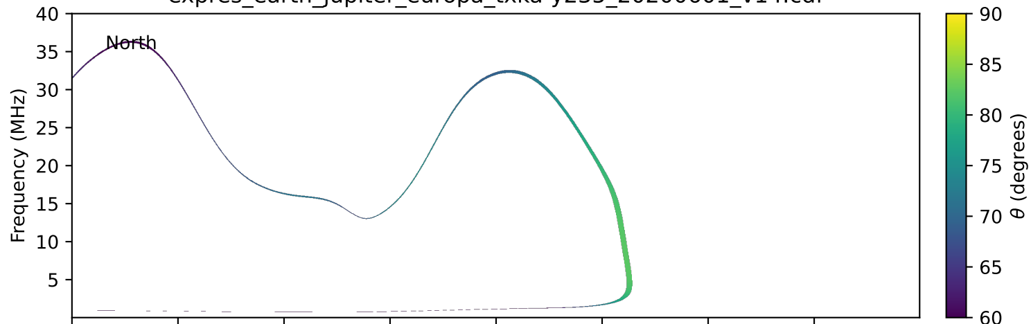
expres_earth_jupiter_europa_txka-y235_20200601_v14.cdf
