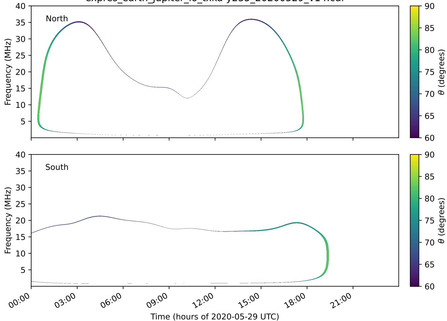
expres_earth_jupiter_io_txka-y235_20200529_v14.cdf
