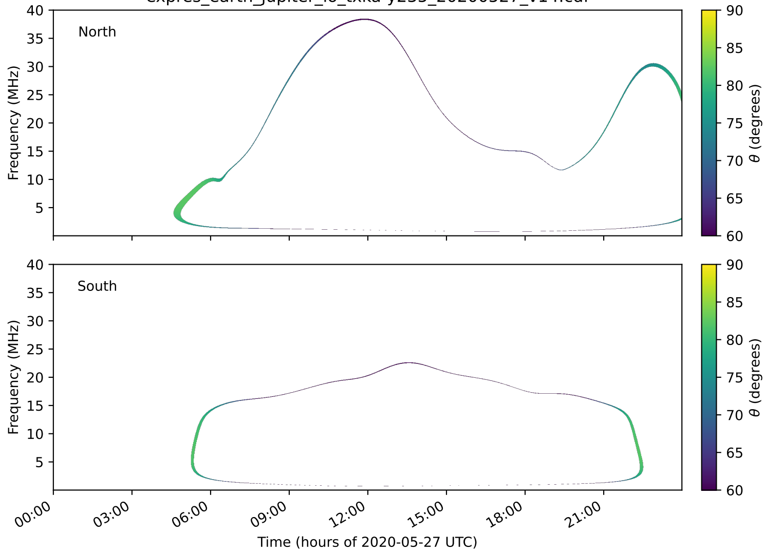
expres_earth_jupiter_io_txka-y235_20200527_v14.cdf
