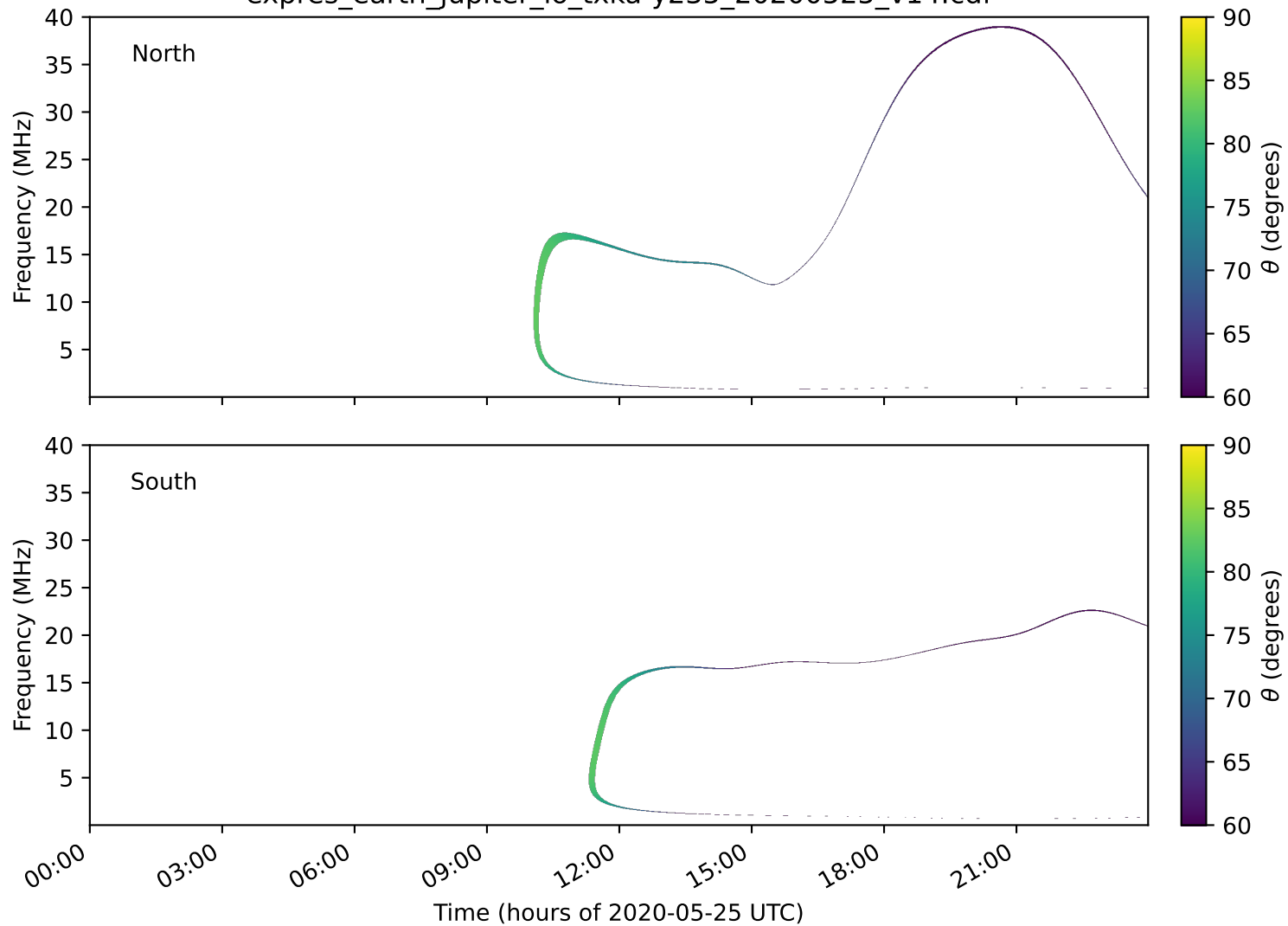
expres_earth_jupiter_io_txka-y235_20200525_v14.cdf
