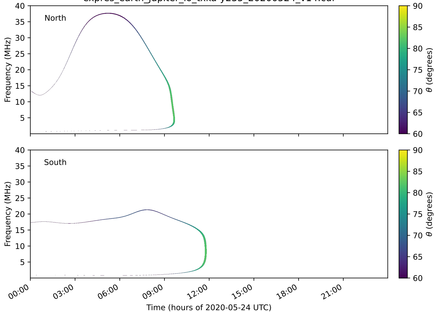
expres_earth_jupiter_io_txka-y235_20200524_v14.cdf
