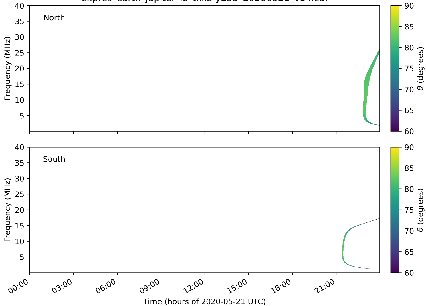
expres_earth_jupiter_io_txka-y235_20200521_v14.cdf
