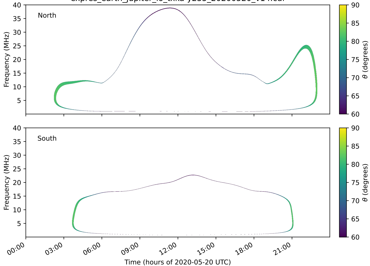
expres_earth_jupiter_io_txka-y235_20200520_v14.cdf
