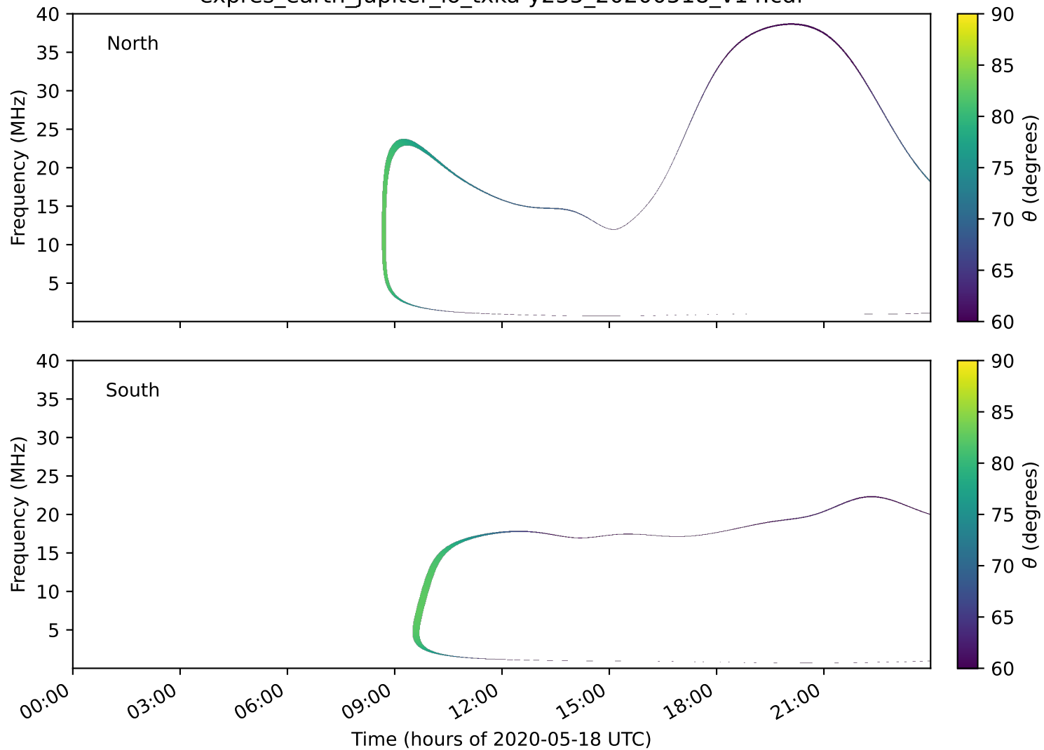
expres_earth_jupiter_io_txka-y235_20200518_v14.cdf
