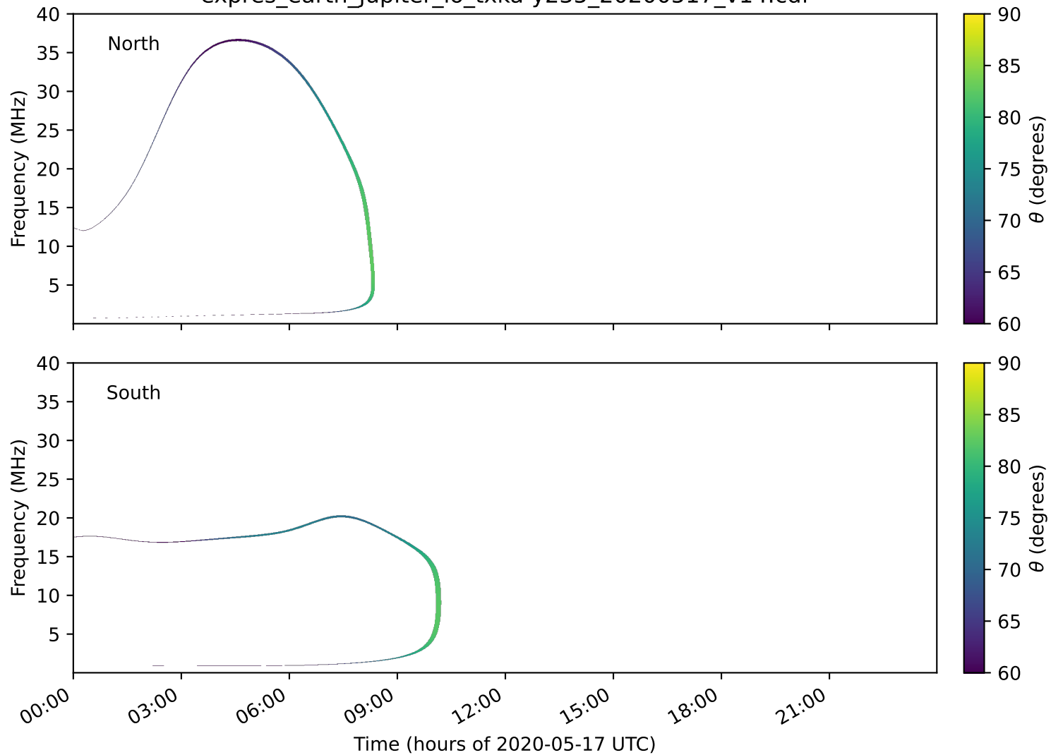
expres_earth_jupiter_io_txka-y235_20200517_v14.cdf
