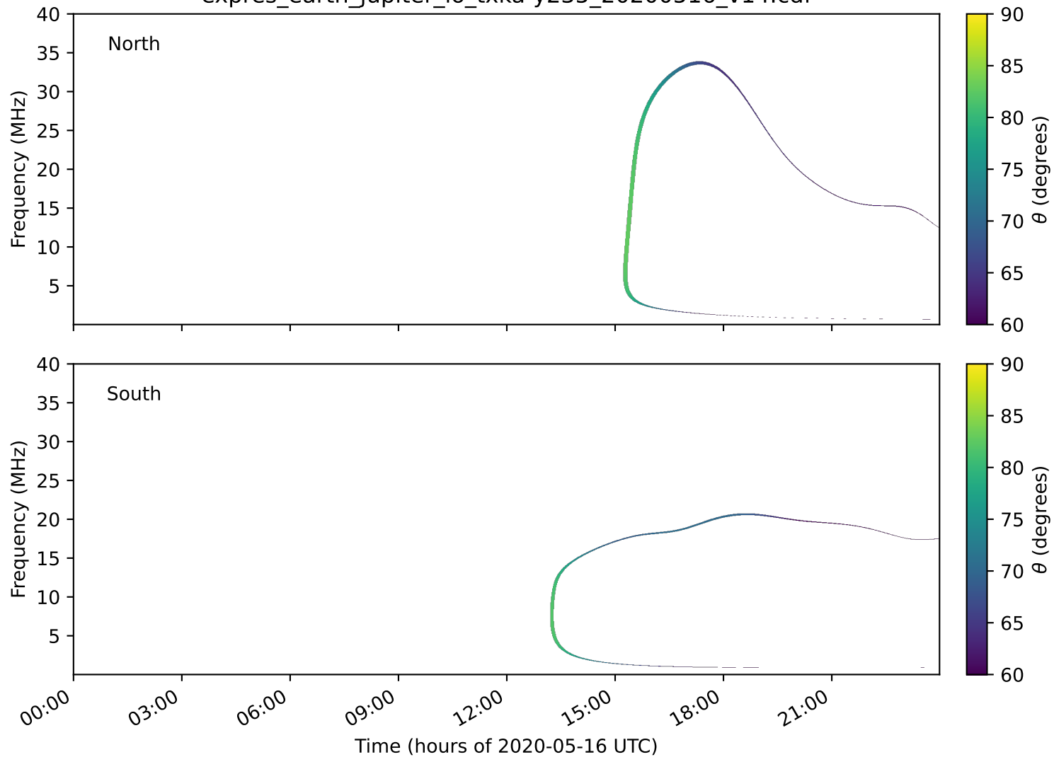
expres_earth_jupiter_io_txka-y235_20200516_v14.cdf
