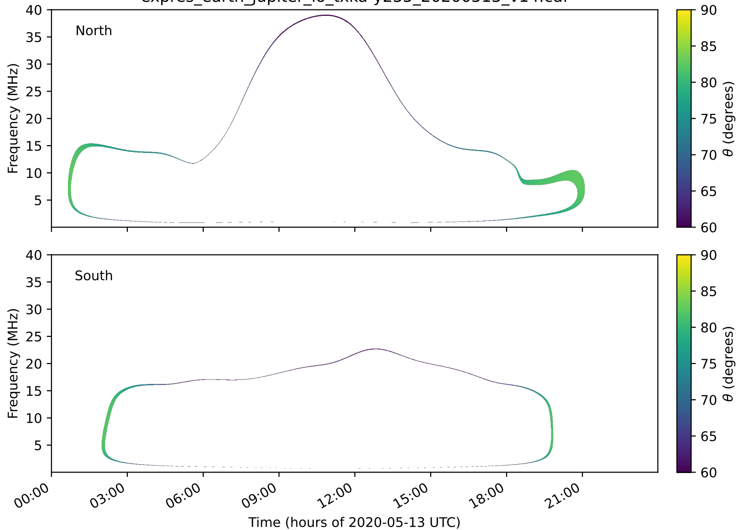
expres_earth_jupiter_io_txka-y235_20200513_v14.cdf
