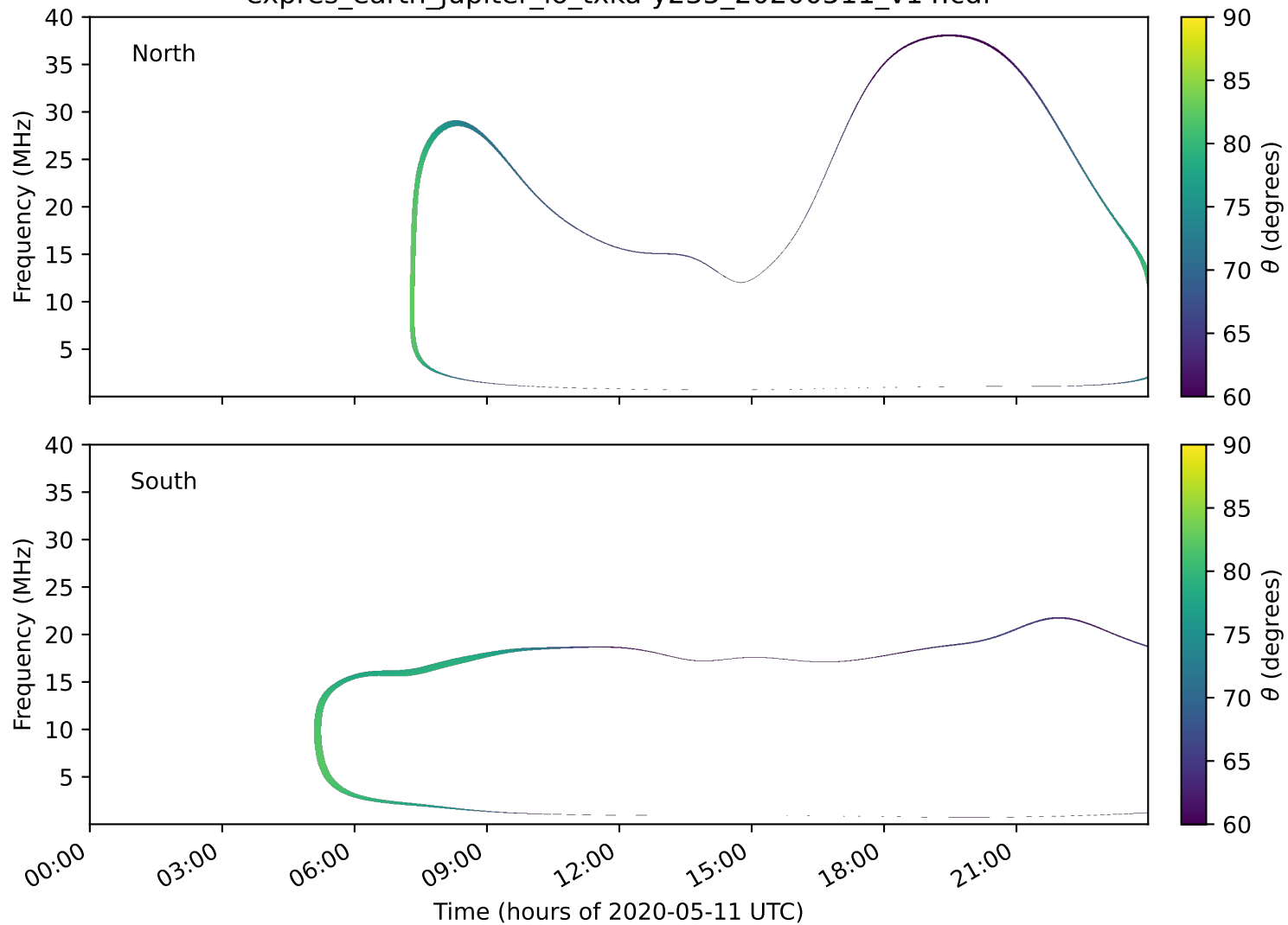
expres_earth_jupiter_io_txka-y235_20200511_v14.cdf
