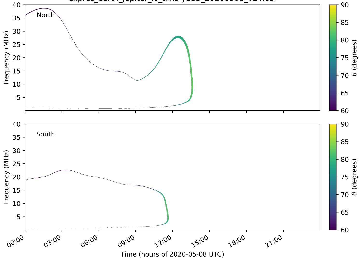
expres_earth_jupiter_io_txka-y235_20200508_v14.cdf
