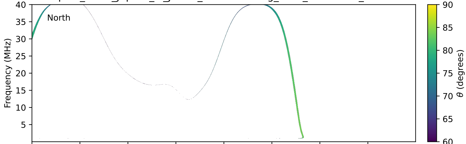
expres_earth_jupiter_io_jrm33_lossc-wid1deg_3kev_20200522_v11.cdf
