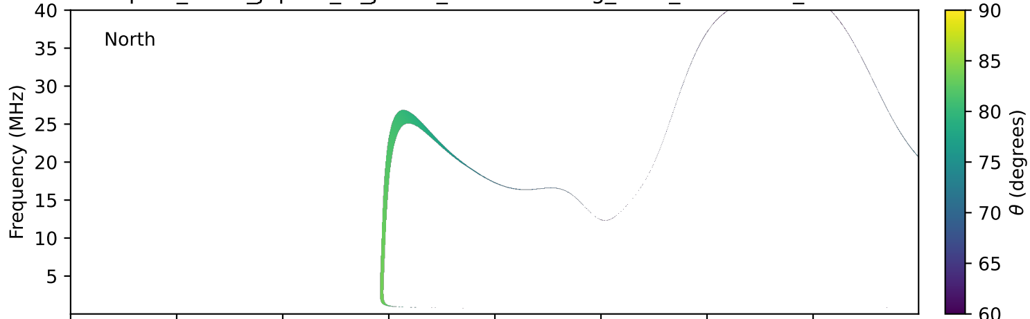
expres_earth_jupiter_io_jrm33_lossc-wid1deg_3kev_20200518_v11.cdf
