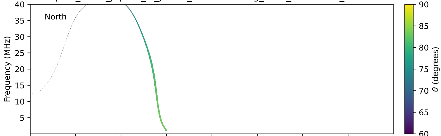
expres_earth_jupiter_io_jrm33_lossc-wid1deg_3kev_20200517_v11.cdf
