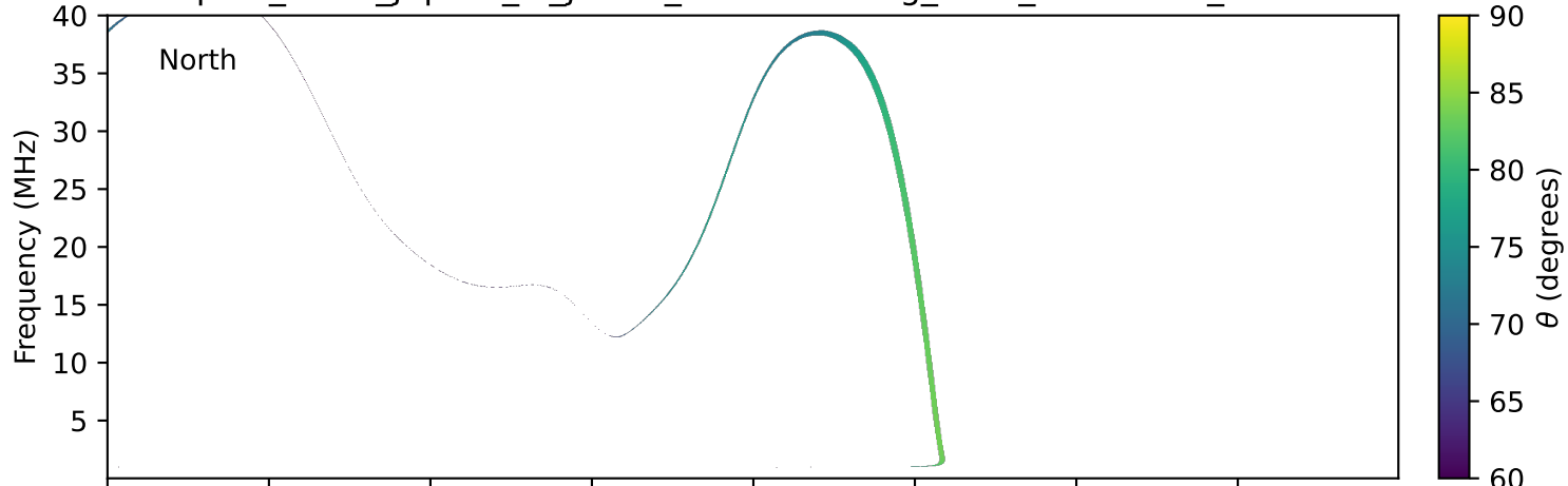
expres_earth_jupiter_io_jrm33_lossc-wid1deg_3kev_20200515_v11.cdf
