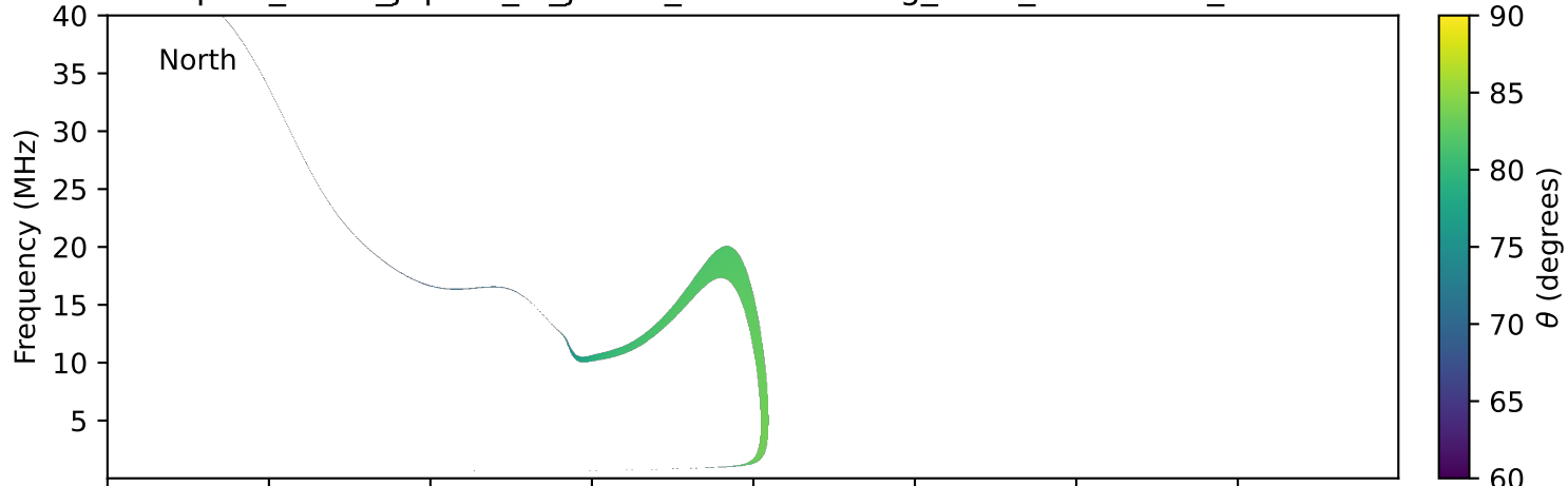
expres_earth_jupiter_io_jrm33_lossc-wid1deg_3kev_20200501_v11.cdf
