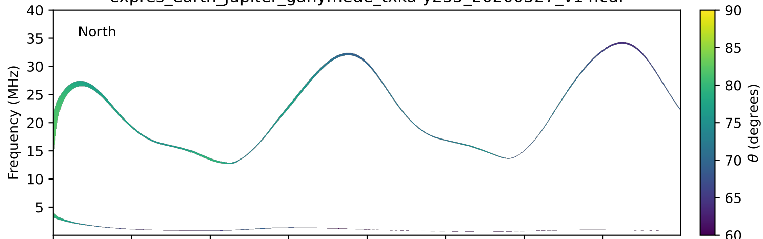
expres_earth_jupiter_ganymede_txka-y235_20200527_v14.cdf
