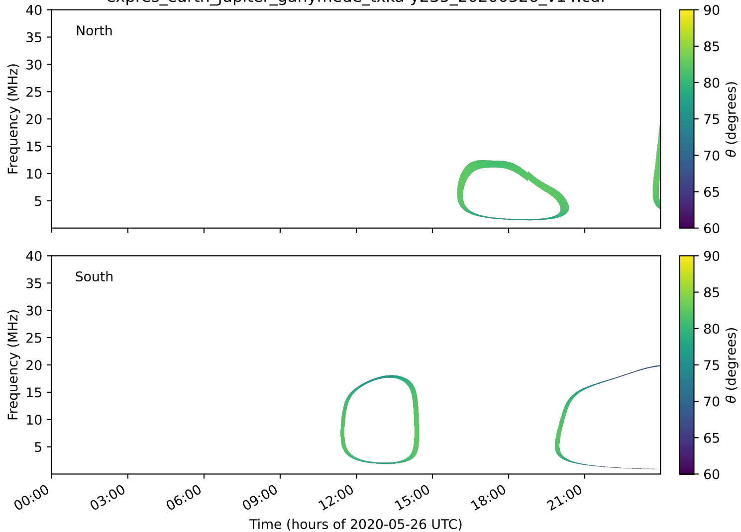
expres_earth_jupiter_ganymede_txka-y235_20200526_v14.cdf
