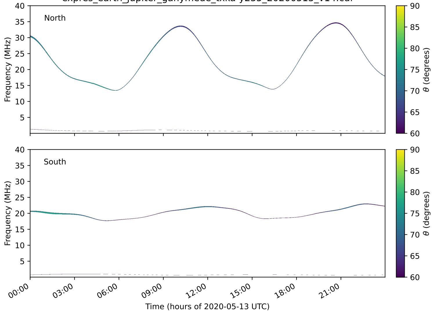
expres_earth_jupiter_ganymede_txka-y235_20200513_v14.cdf
